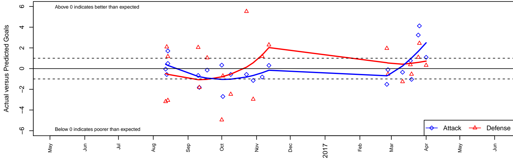
Central WA SA Navy B03 Dots are actual minus expected GF (blue circles) and GA (red triangles). Blue line is smoothed change in attack strength. Red is smoothed change in defense strength.
